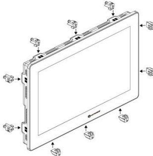
USP-156-xxx: 10 mounting brackets
