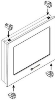
USP-070-xxx: 4 mounting brackets
